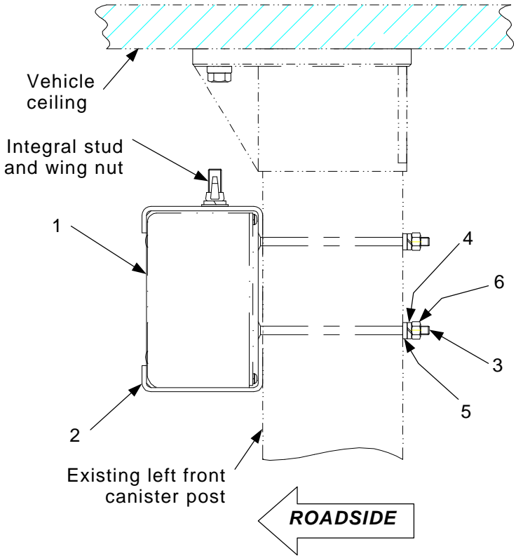
Figure 4-5. Loudspeaker Installation
